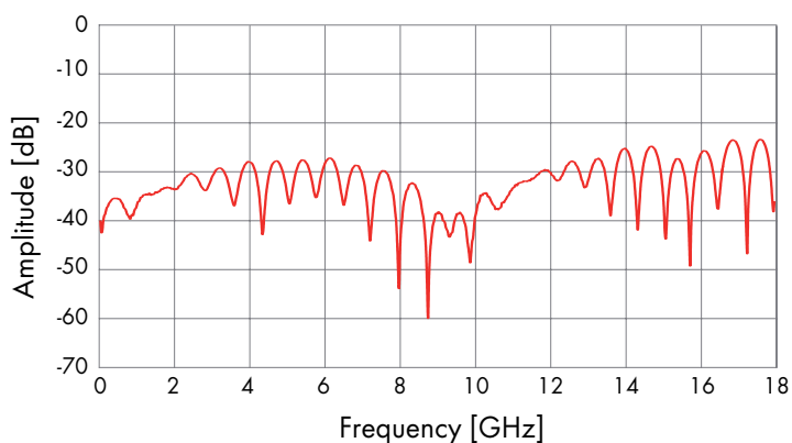
Typical return loss value assembly
